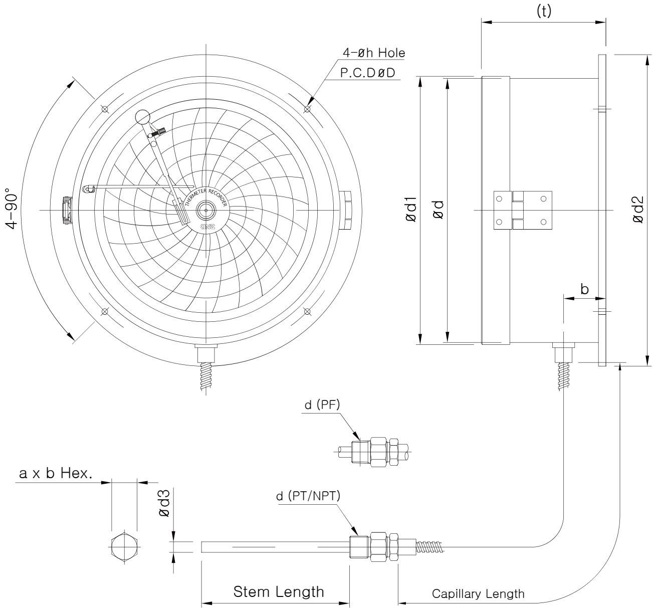
Model. DS-2031
